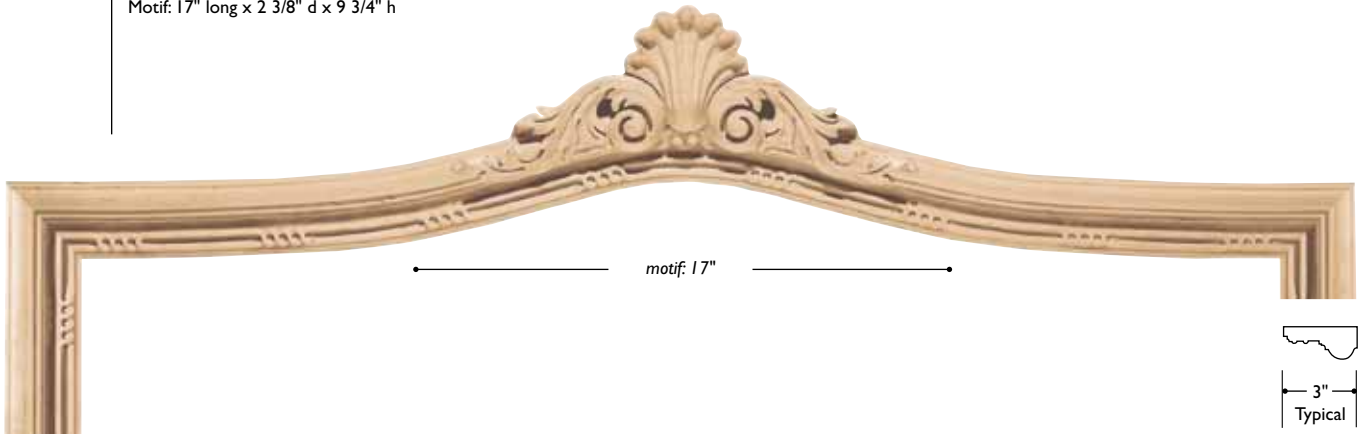
CRW-SC3 Crown Shell Curved Small - 50" long Motif: 17" long x 2 3/8" d x 9 3/4" h
