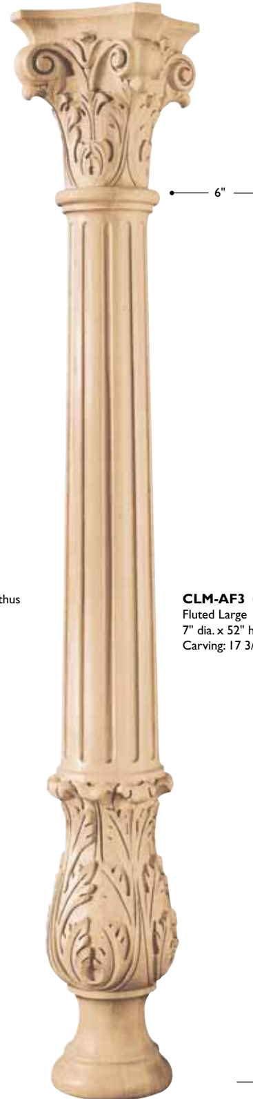
CPL-CR3 Capital Corinthian Round Large - 10" h Top: 9 1/4" sq. Bottom: 5" dia. Sold separately
