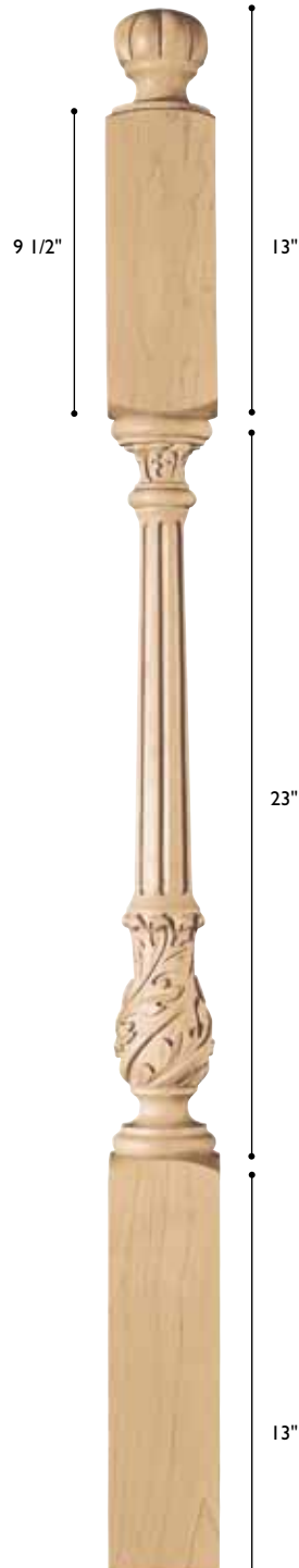
NWL-AF3 Newel Acanthus Fluted Large 49" h Top: 3 1/2" sq. Bottom: 3 1/2" sq.
