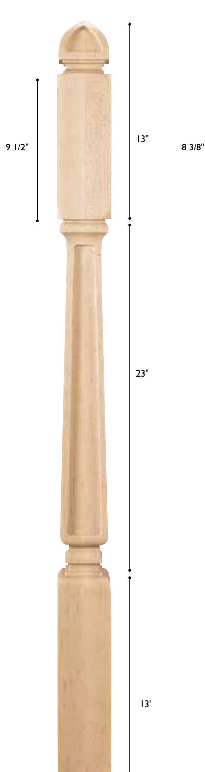
NWL-AMA-XX-6XXX Newel American Arts and Crafts Large 49" h Top: 3 1/2" sq. Bottom: 3 1/2" sq.
