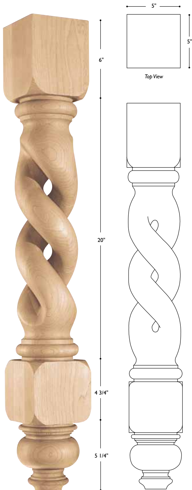
PST-MAB-TW-5XXX Post Monarch Bay Twist Medium 36" h x 5" w x 5" d
