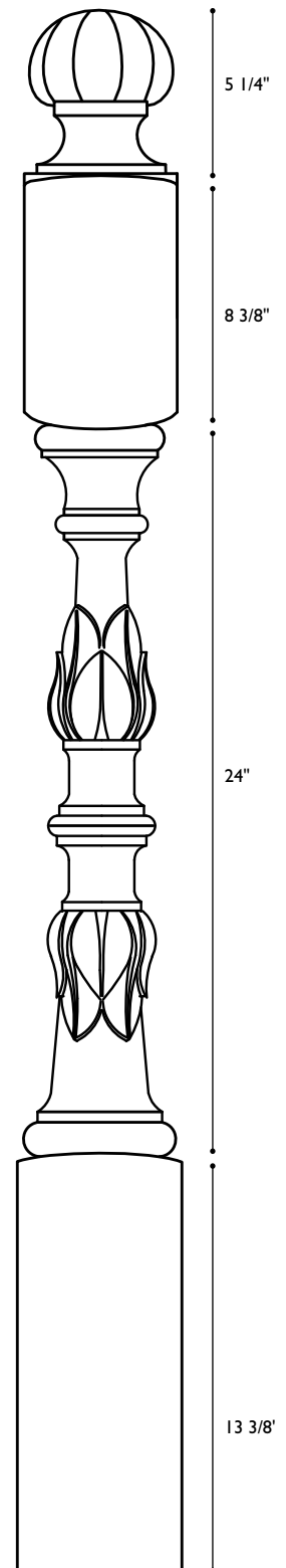
NWL-ALB-5 Newell Hearst Alabaster X-Large 51" h Top: 5" sq. Bot: 5 3/8" sq.
