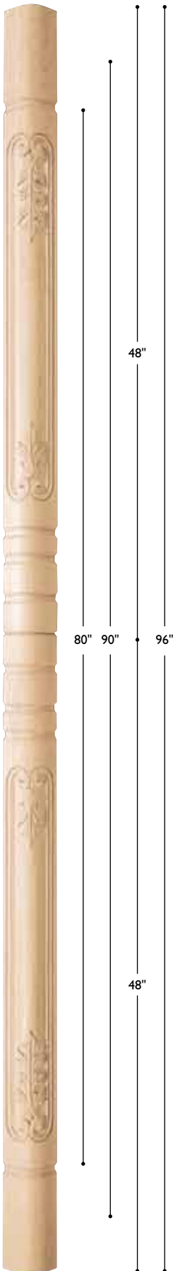
PST-AC4 (x2) Post Acanthus Corner 96" h x 3" w x 3" d Assembly required
