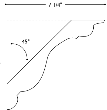
Crown Profile
