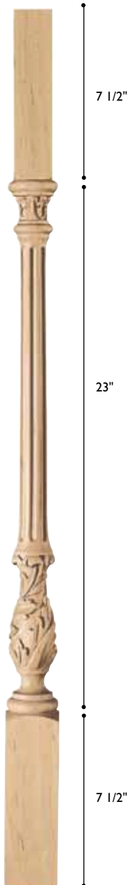
BLR-AF2 Baluster Acanthus Fluted Medium 38" h Top: 1 3/4" Bottom: 2 3/8" sq.
